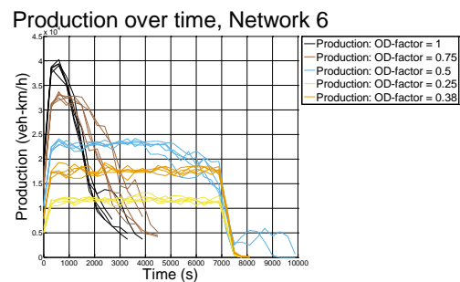
Figure 7.12: Production over time, network 6
