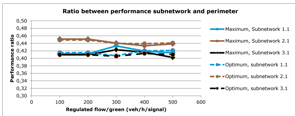
Figure 8.8: Performance ratio subnetwork/perimeter for network 1, 2 and 3
