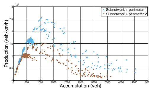
Figure 3.4: Production vs. Accumulation subnetworks and perimeters
