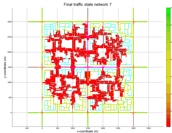
Figure 7.6: Gridlock state network 7
