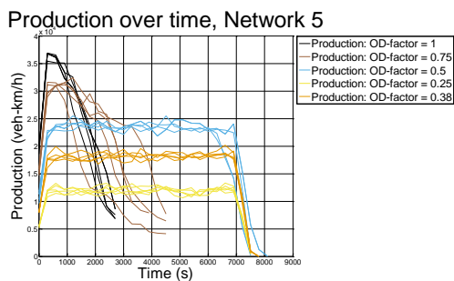
Figure 7.11: Production over time, network 5
