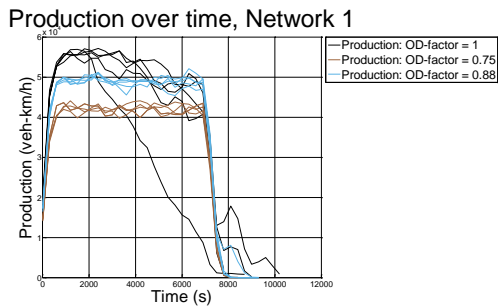
Figure 7.7: Production over time, network 1
