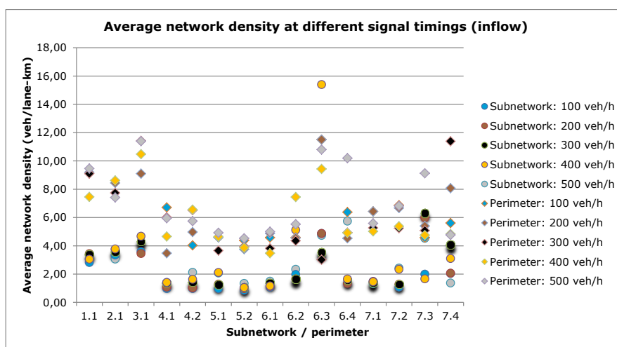
Figure 8.12: Optimal network density at different signal timings (controlled inflow) 22
