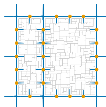
Figure 4.3: Network with single asymmetrical arterial
