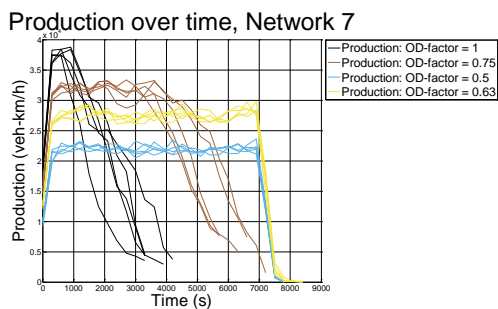
Figure 7.13: Production over time, network 7
