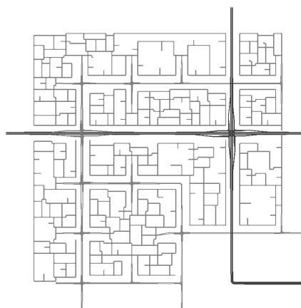
Figure 5.12: Network in VISSIM
