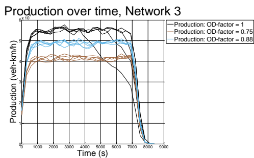
Figure 7.9: Production over time, network 3
