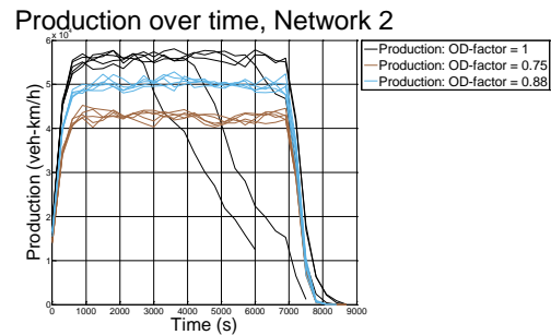
Figure 7.8: Production over time, network 2
