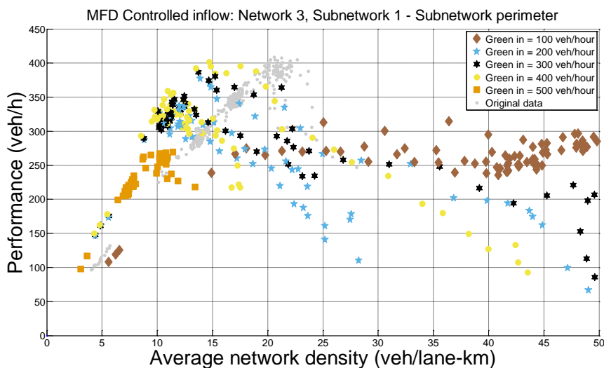
Figure 8.2: MFD of subnetwork perimeter network 3 – Controlled inflow
