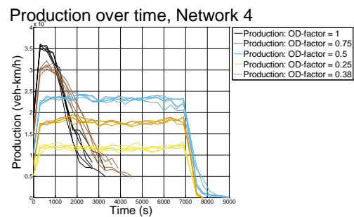
Figure 7.10: Production over time, network 4
