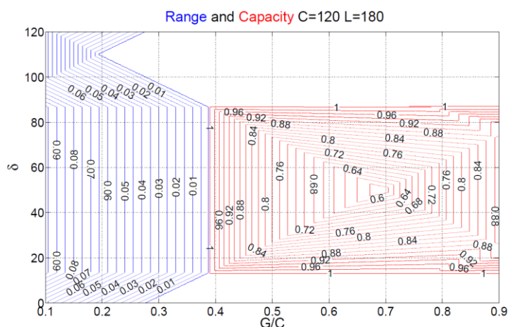
Figure 2.9: Effect of different signal timings on network capacity (Boyaci and Geroliminis, 2010)
