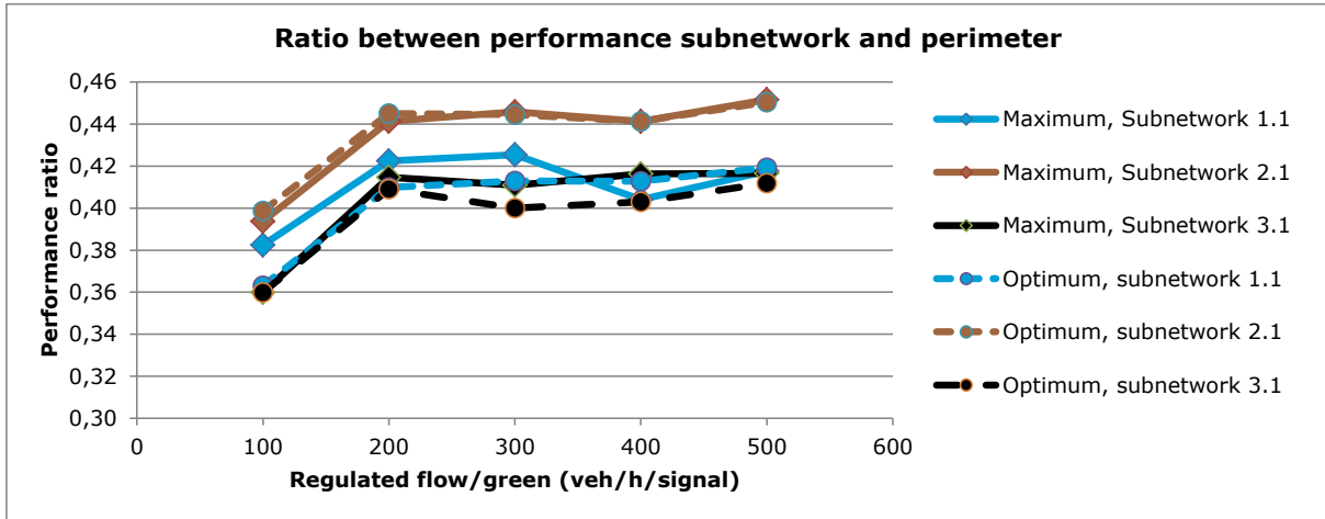
Figure 8.1: Performance ratio subnetwork/perimeter, network 1, 2 and 3
