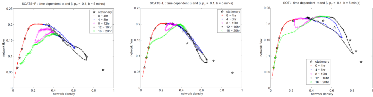
Figure 2.11: MFDs for the time-dependent isotropic demand scenario (Zhang et al., 2011) From left to right: SCATS-F, SCATS-L, SOTL
