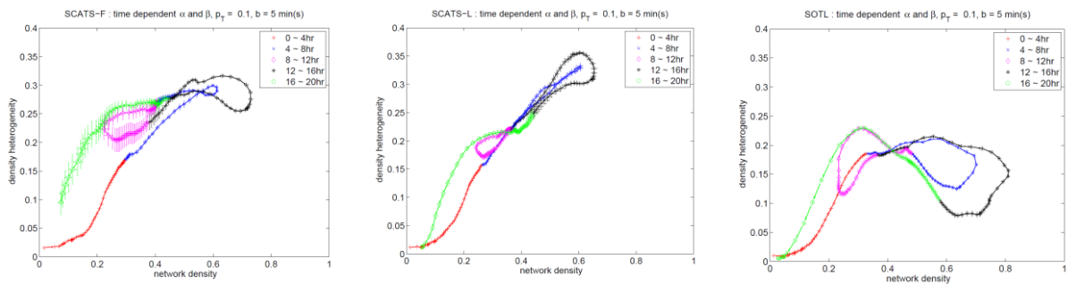
Figure 2.12: Variation of density, belonging to the MFDs in Figure 2.11 (Zhang et al., 2011) From left to right: SCATS-F, SCATS-L, SOTL
