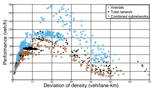
Figure 3.11: Performance vs. Deviation of density
