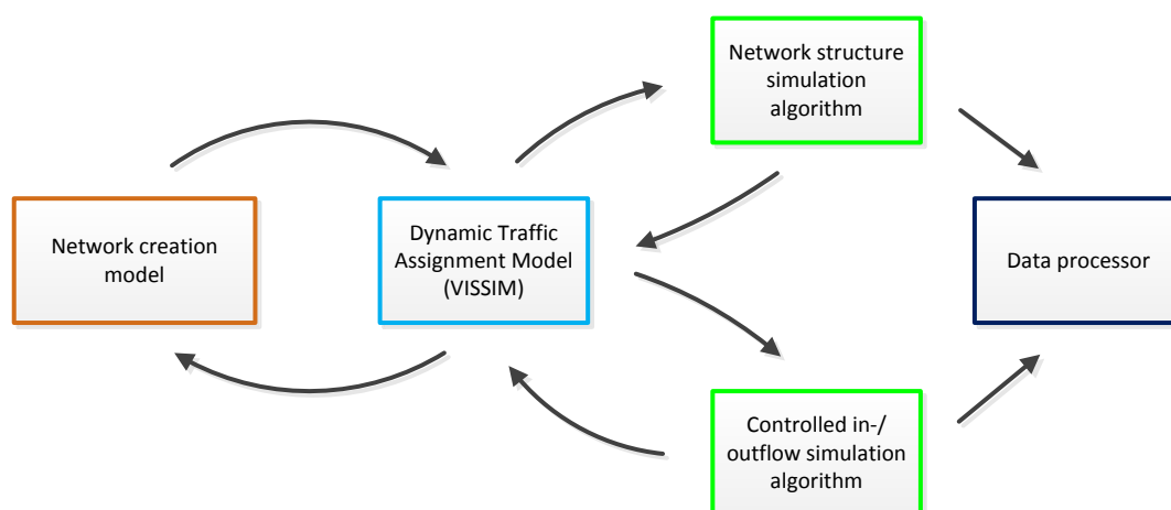
Figure 5.1: General framework
