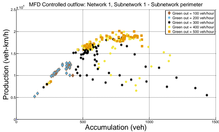
Figure 8.14: Example of differences in optimal accumulations under different signal settings
