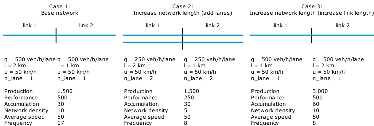
Figure 3.14: Effect of increasing network length by adding additional lanes or lengthening links
