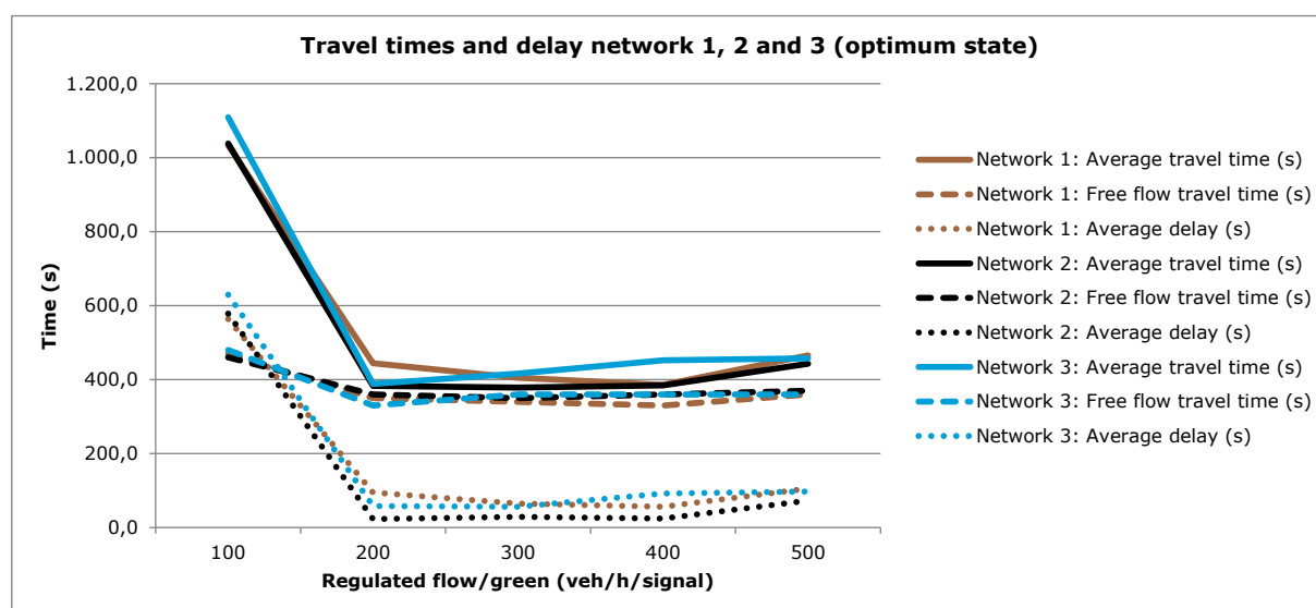
Figure 8.3: Travel times and delay for network 1, 2 and 3 (optimum state)
