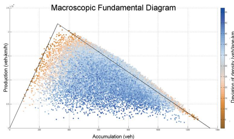
Figure 3.19: Deviation of density vs. Production and Accumulation with envelope
