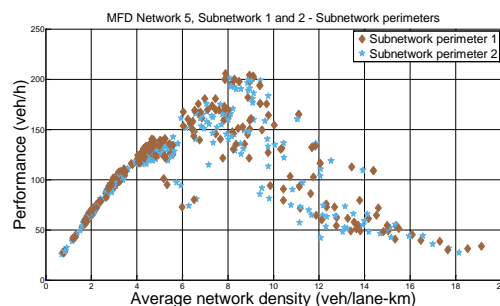
Figure 7.22: Comparison of perimeter MFDs network 5
