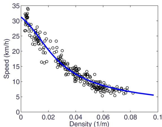
Figure 2.10: Fundamental velocity-density relationship for a central area of Yokohama. Small circles correspond to empirical data by Kuwahara as evaluated by Daganzo and Geroliminis (2008). The blue curve is fitted using equations (2.9) – (2.12). (Helbing, 2009)
