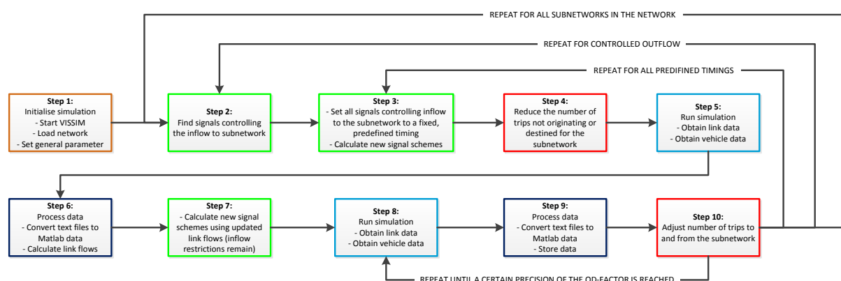
Figure 5.15: Simulation algorithm to evaluate the effect of signal settings.
