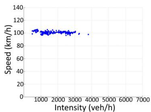
Figure A.12 – Intensity-density diagram, 1 February 2016, A4 hmp 57.35
