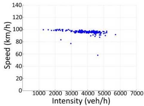
Figure A.14 – Intensity-density diagram, 5 February 2016, A13 hmp 15.4
